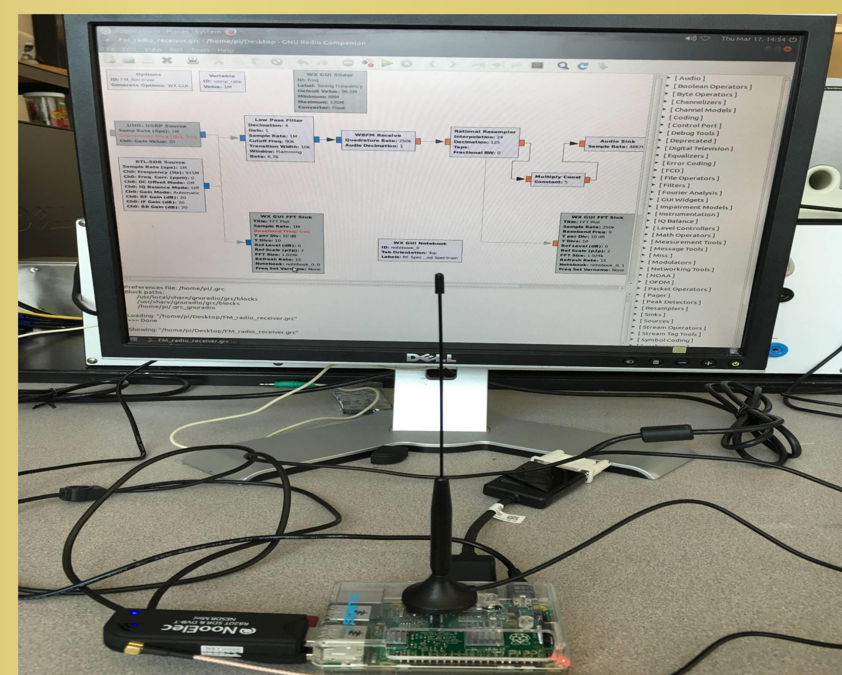
Fig.(2): Community radio receiver.
