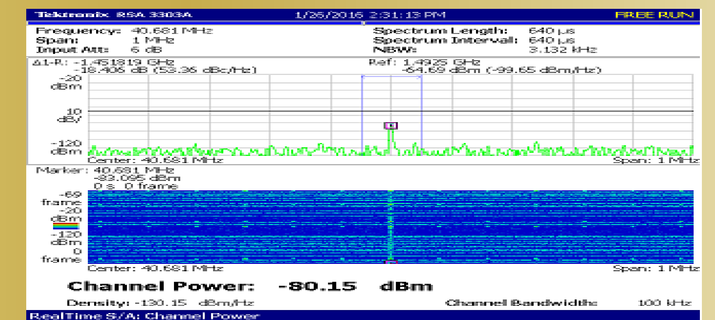
Fig.5: RSA 3303A real time spectrum analyzer snapshot.
