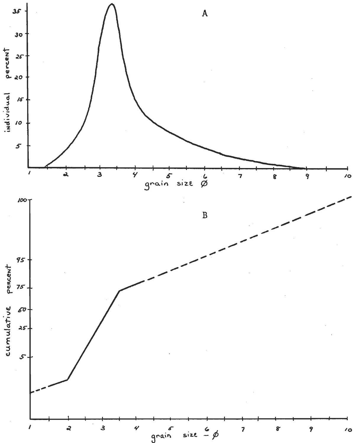
Figure 9. Curves obtained from grain size analysis of the Schmidt Site sediment. A) Frequency curve B) Cumulative percent curve drawn on probability paper,
