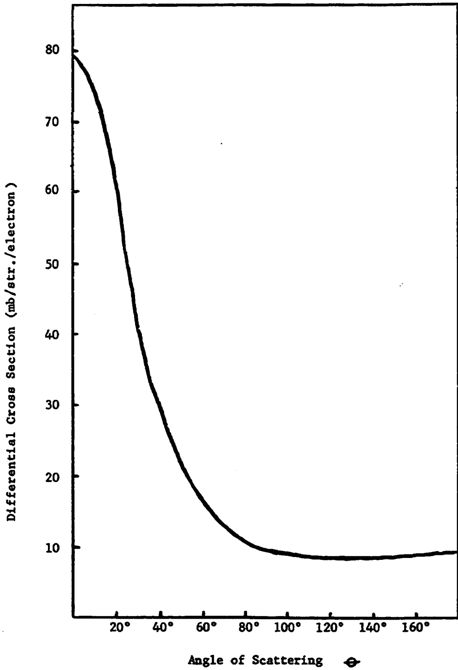
Figure I. Compton Cross Section vs. Angle
